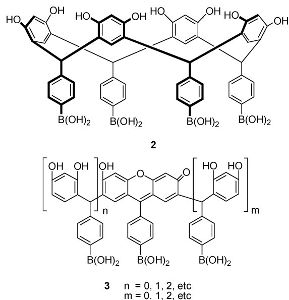
Figure 3. Structures of the resorcinarene boronic acid 2 and its chromophoric products ( 3 ) formed in situ.
