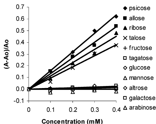
Figure 7. Plots of relative absorbance changes vs concentration of 11 monosaccharides in solutions comprised of phosphate buffer (0.1 mL, 60 mM, pH = 7.4) added to 1 (0.07 mM) in DMSO (0.9 mL) and 2 (1.9 mM) monitored at 560 nm.
