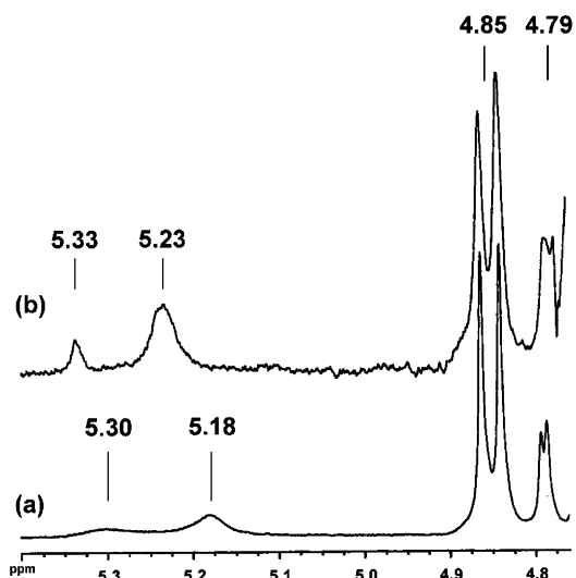
Figure 5. Expansion of the ^1\text{H} NMR spectra of solutions of (a) D-ribose and (b) a mixture of 1 and D-ribose (0.15 M NaOD/D 2 O). The resonances shown correspond to the anomeric protons of each of the four cyclic forms. The assignments are \delta (ppm): 5.30 ( \alpha -ribofuranose), 5.18 ( \beta -ribofuranose), 4.85 ( \beta -ribopyranose), and 4.79 ( \alpha -ribopyranose). Upon the addition of 1 only the resonances corresponding to the ribofuranoses exhibit a downfield shift. This is expected as a result of cyclic boronate formation with ribofuranose (ref 3c).
