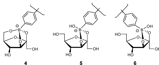
Figure 12. Anionic fructofuranose-boronate ester structures.
