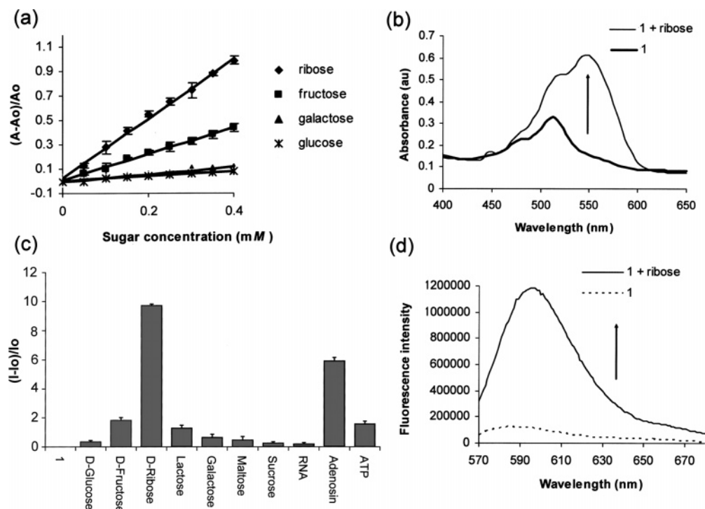
Figure 1. (a) Relative absorbance changes vs concentration of various monosaccharides in phosphate buffer (0.1 mL, 60 mM, pH 7.4) added to 1 ( 7.2 \times 10^{-5} M) in DMSO (0.9 mL) and monitored at 560 nm. (b) The UV-vis spectra of a solution of 1 ( 7.2 \times 10^{-5} M) alone and 1 with added ribose ( 4 \times 10^{-4} M). (c) Relative fluorescence emission spectra at 597 nm of 1 ( 4 \times 10^{-9} M) and saccharides and saccharide-containing molecules ( 1.85 \times 10^{-3} M) in 9:1 DMSO/phosphate buffer (0.05 M, pH 7.4) excited at 565 nm. (d) Fluorescence emission spectra of a solution of 1 ( 4 \times 10^{-9} M) and 1 with added ribose ( 1.85 \times 10^{-3} M) in 9:1 DMSO/phosphate buffer (0.05 M, pH 7.4) excited at 565 nm.
