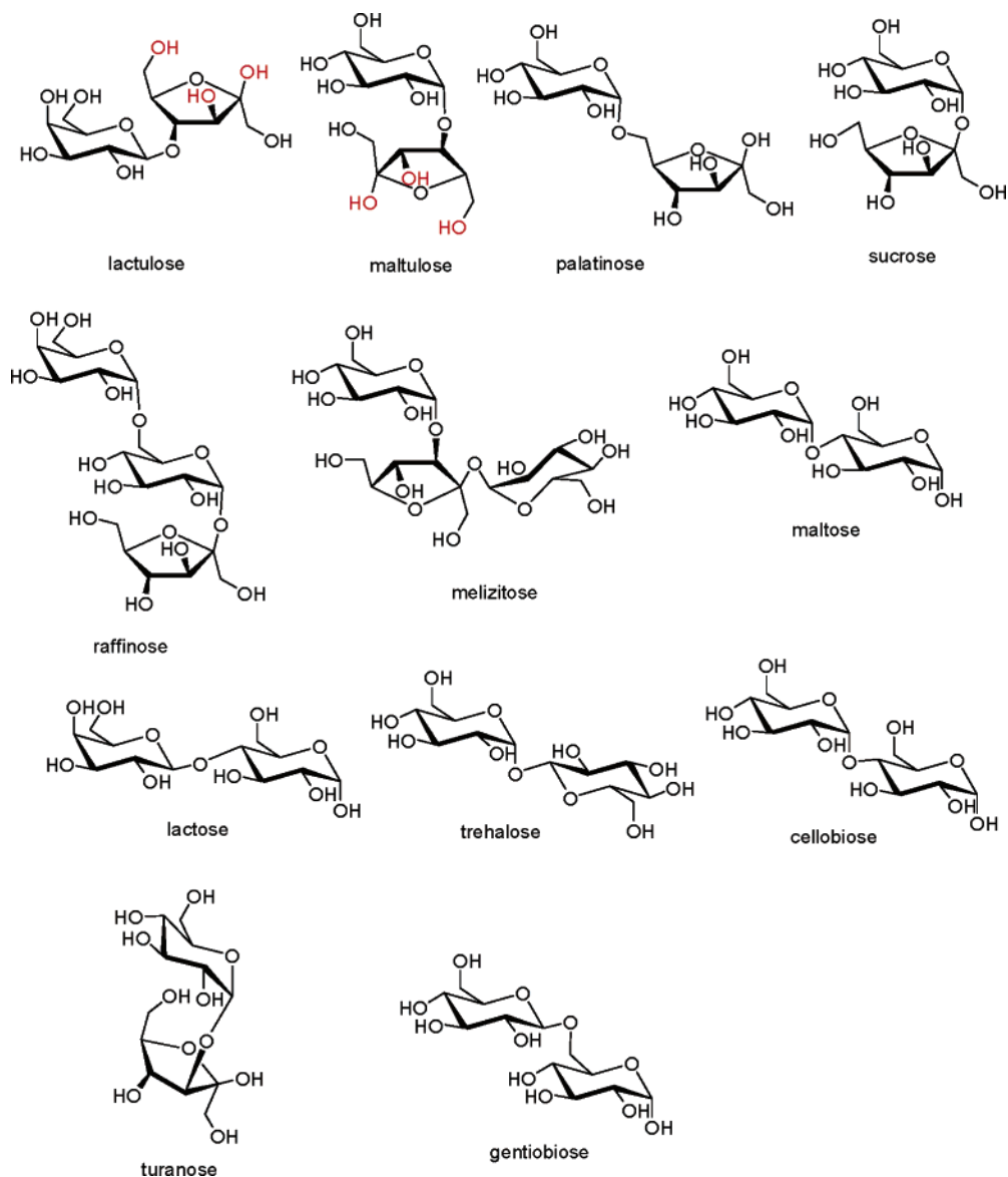
Figure 13. Di- and trisaccharides studied.
