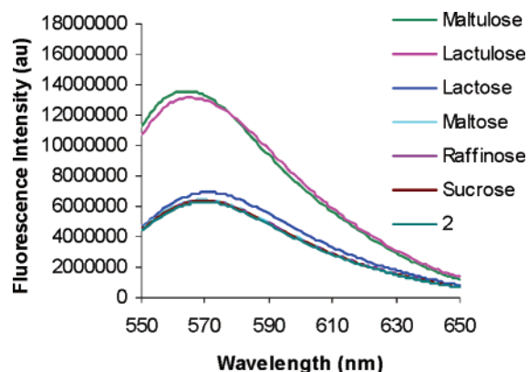
Figure 14. Fluorescence emission spectra of a solution of 2 ( 1 \times 10^{-3} M) and 2 with added di- and trisaccharides ( 1.85 \times 10^{-3} M), all in 9:1 DMSO/phosphate buffer (0.05 M, pH 7.4) excited at 535 nm. This result shows the selectivity for lactulose and maltulose. The other di- and trisaccharides tested afford no detectable signal. Only lactulose and maltulose can adapt the proper terminal residue configurational preference (Figure 13). The selectivity is confirmed by UV-vis spectroscopy (Supporting Information).
