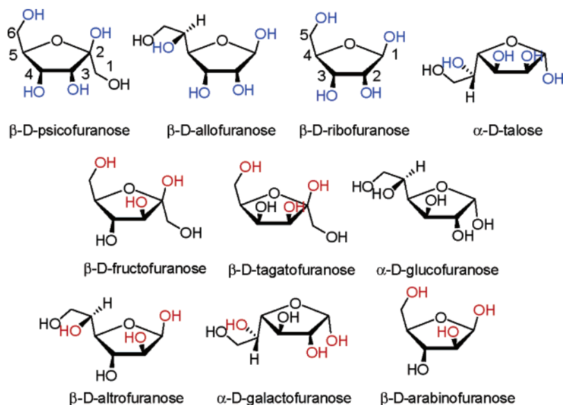
Figure 6. Structures of 11 monosaccharides in their furanose forms. Compound 1 is selective for sugars with hydroxyls shown in blue. Compound 3 is selective for sugars with hydroxyls shown in red.
