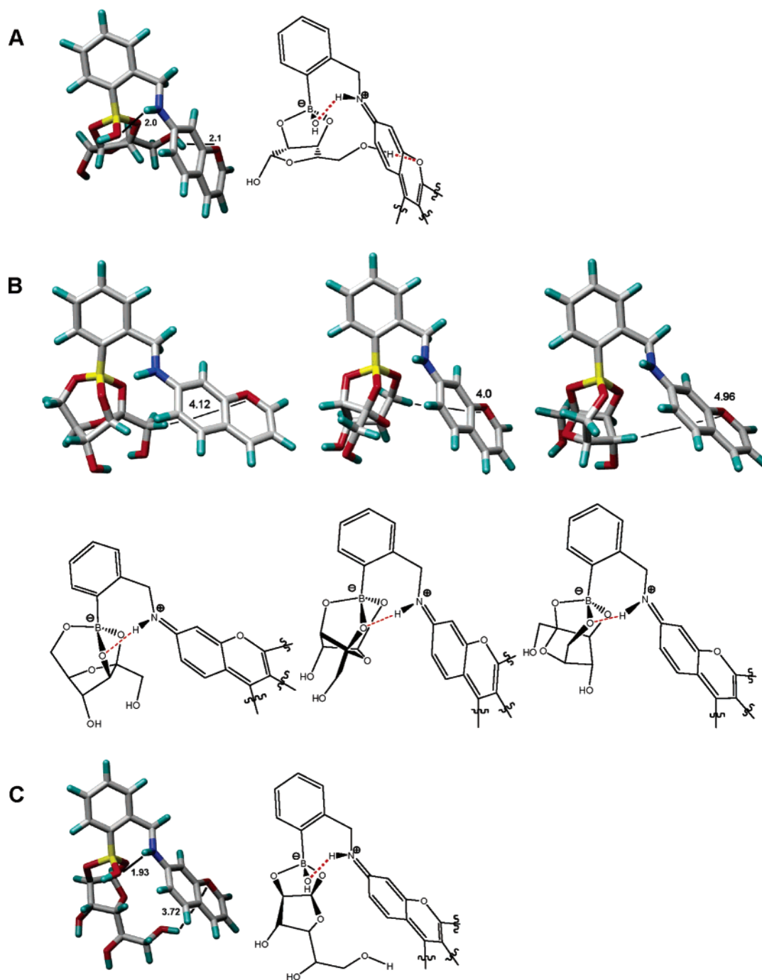
Figure 9. Energy-minimized structures of boronates derived from 1 and ribofuranose (“endo” isomer, structure A), fructofuranose (three rotamers, structures B), and glucofuranose (“exo” isomer, structure C; the complementary conformers of the ribo- and glucofuranose boronates are included in the Supporting Information). A subunit of the rhodamine chromophore moiety is shown for clarity and used in the simulations in order to simplify the calculations. The above-calculated structures show that the ribofuranose complex exhibits the relatively best geometry for promoting direct contacts between the bound sugar moiety and the chromophore moiety of 1 . Studies aimed at evaluating the specific interactions between ribose, adenosine, ribosides, and ribotides with 1 that might involve \pi - \pi stacking, \sigma - \pi interactions, and/or charged hydrogen bonding between the sugar and the rhodamine carboxylate functionality are ongoing.
